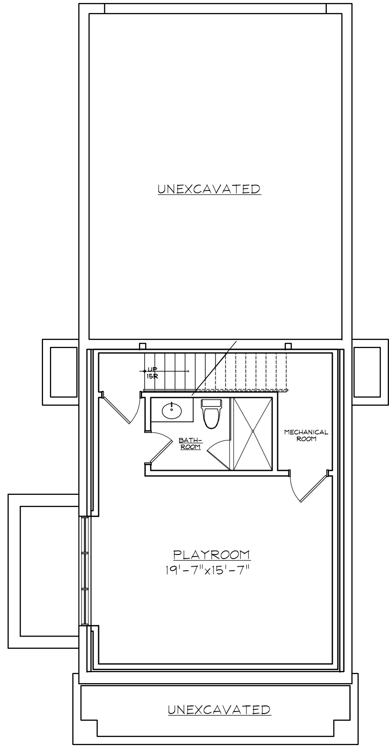
BASEMENT PLAN (2-24-14) HALSEY LANE REC. PAVILION
