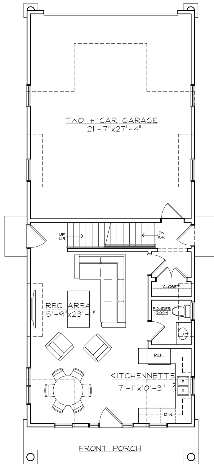
FIRST FLOOR PLAN (2-24-14) HALSEY LANE REC. PAVILION
