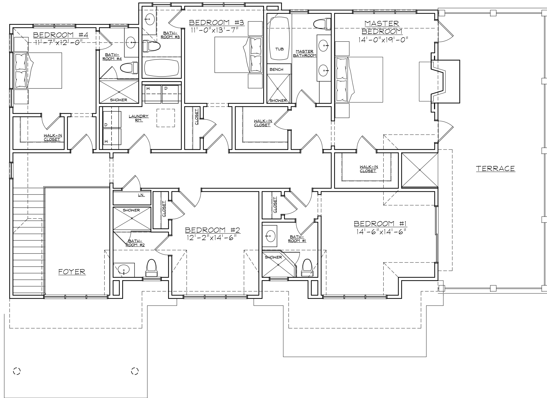
SECOND FLOOR PLAN (2-24-14) HALSEY LANE 2,102 SQ. FT.
