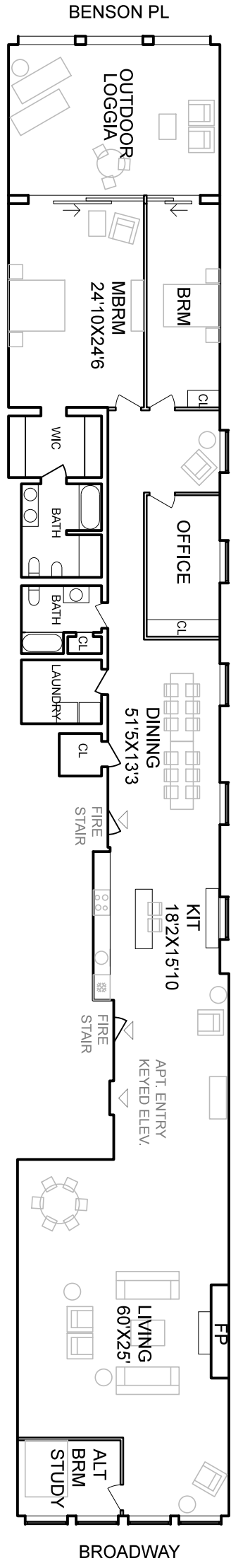
2 ALT PLAN 1/16"=1'-0"
